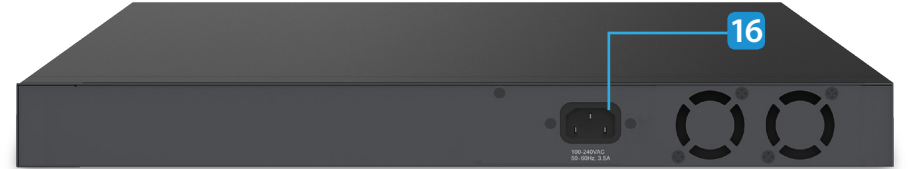
EGS7228P - Back
