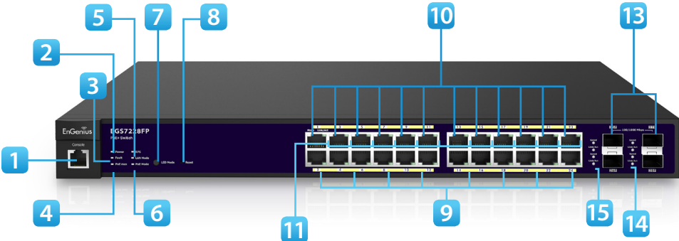
EGS7228FP - Front
